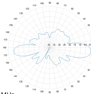
1755 MHz
