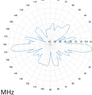
3450 MHz
