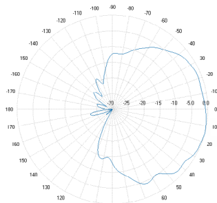
850 MHz
