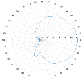
660 MHz
