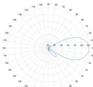
1970 MHz
