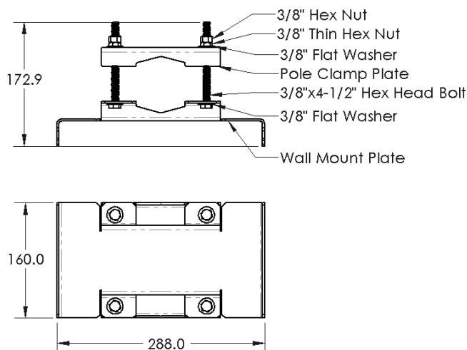
Figure 1. Mounting Bracket
