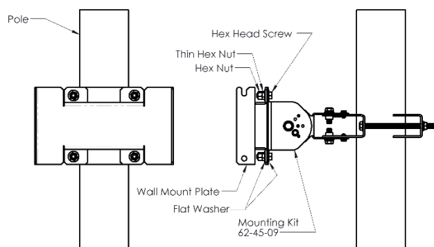
Figure 3. Pole Mount with Tilt
