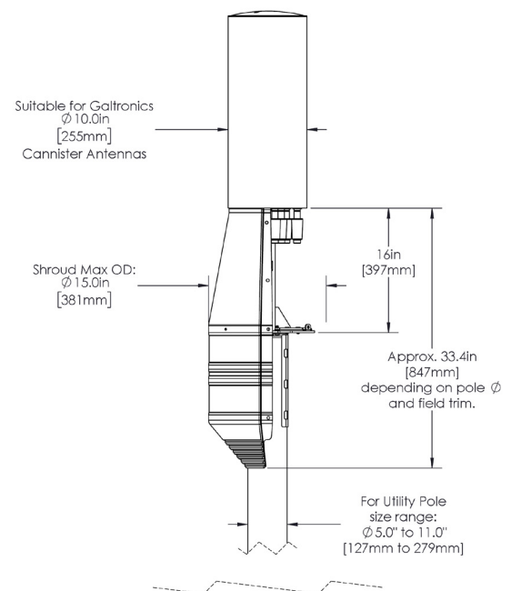
Outline Dimensions
