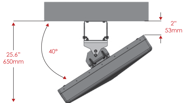
Tilt & Rotation Module. Rotation up to \pm 40^\circ
