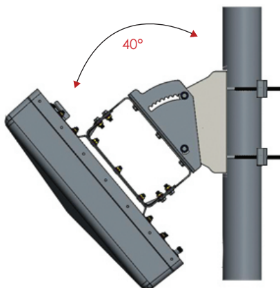
Pole Tilt & Rotation Module. Tilt up to \pm 40^\circ
