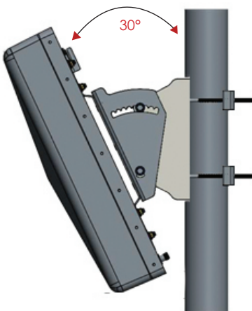
Pole Tilt Module Only. Tilt up to \pm 30^\circ
