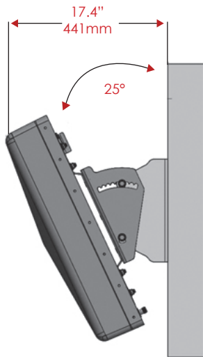
Tilt Module Only. Tilt up to \pm 25^\circ
