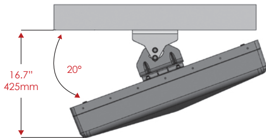
Rotation Module Only. Rotation up to \pm 20^\circ
