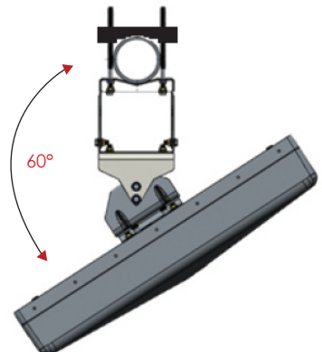
Pole Tilt & Rotation Module. Rotation up to \pm 60^\circ
