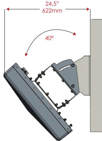
Tilt & Rotation Module. Tilt up \pm 40^\circ
